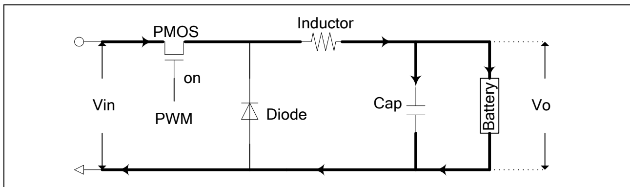
Figure 3 . Buck Converter Switch on
