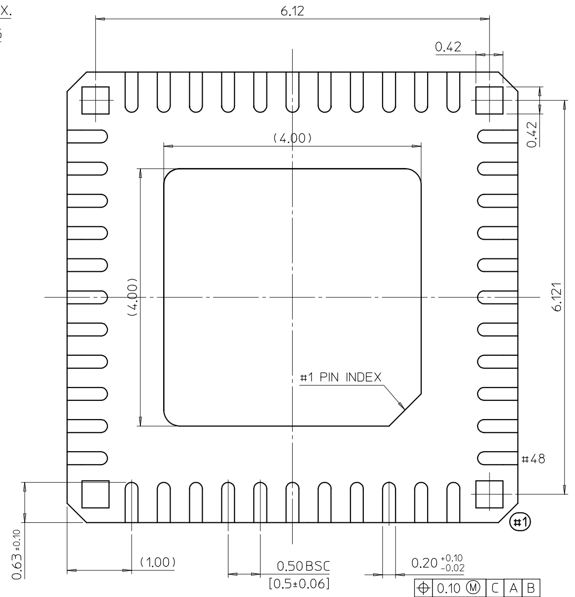
BOTTOM VIEW
