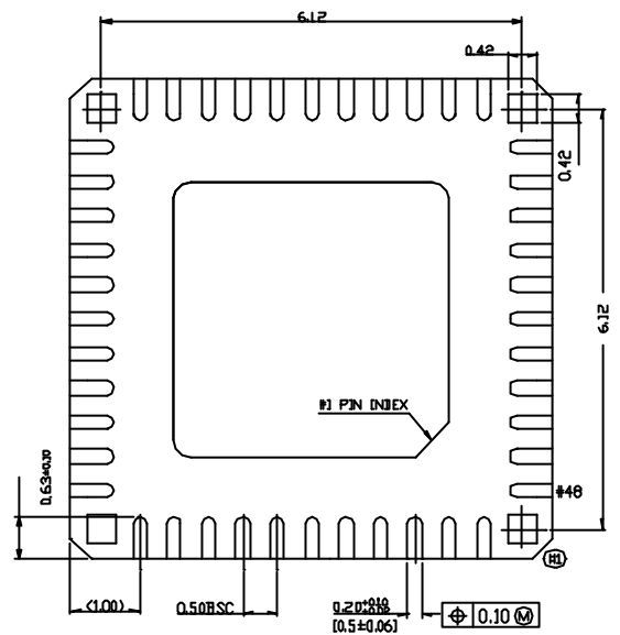
BOTTOM VIEW
