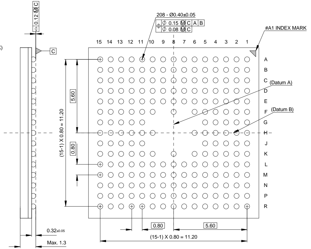
SIDE VIEW
