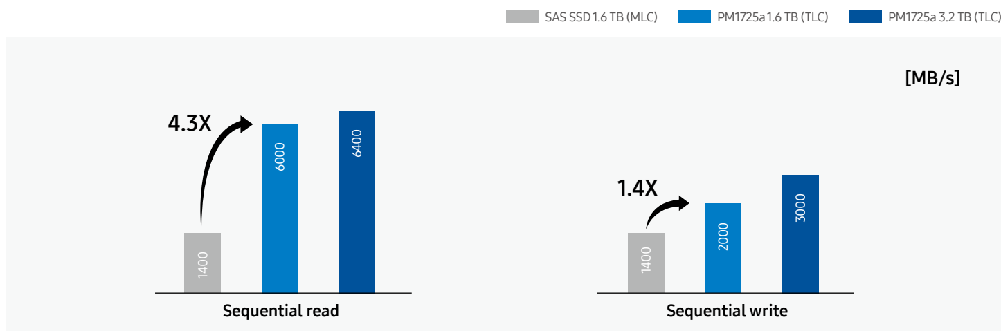
Figure 1. Sequential R/W performance comparison between an MLC SAS SSD and the 1.6 and 3.2 TB TLC PM1725a
